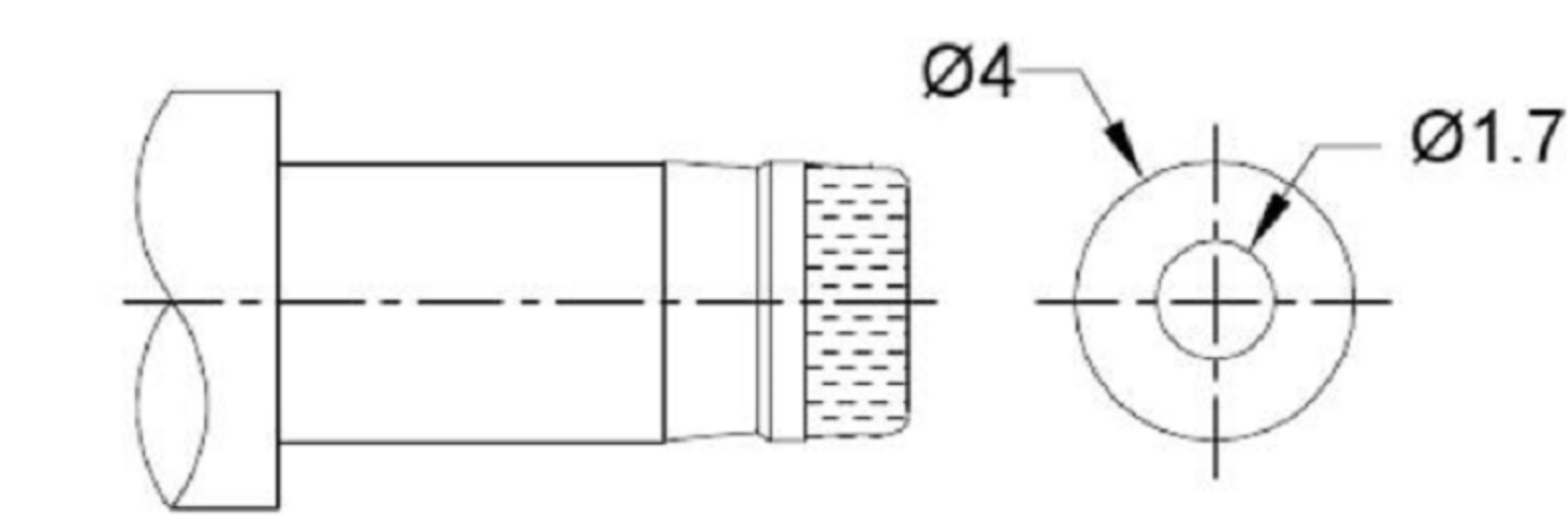
MATING PLUG Jack Insertion Depth: 8.0mm
